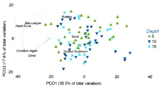
Fig. 3. Principal Coordinate Ordination to compare similarities in benthic/substrate composition between depths. Overlaid vectors represent individual benthic taxa/substrates that have a Pearson's correlation of greater than 0.4 with either of the PCO axes. See Figure 1 for site abbreviations.
