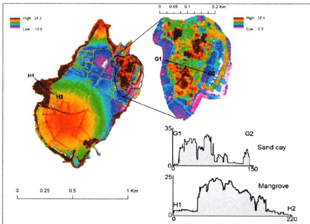
Fig. 9. Digital elevation model of Sabangko showing the full reef flat (left) and the sand cay (inset, right) illustrating profiles of the sand cays, mangroves and shingle ridges.
