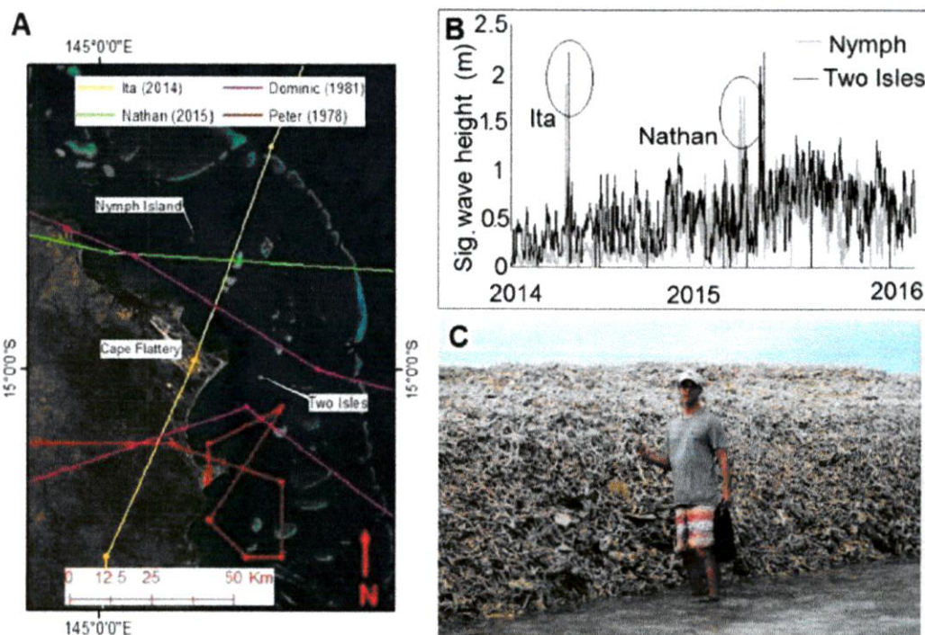
Fig. 10. A. Regional cyclones crossing close to the Great Barrier Reef study sites of Nymph Island and Two Isles throughout the period for evaluation of reef flat change to mangroves and sand cays, B. Significant wave heights measured at Nymph Island and Two Isles for the passages of Cyclones Ita and Nathan, C. Shingle ridge observed on the windward side of Nymph reef.
