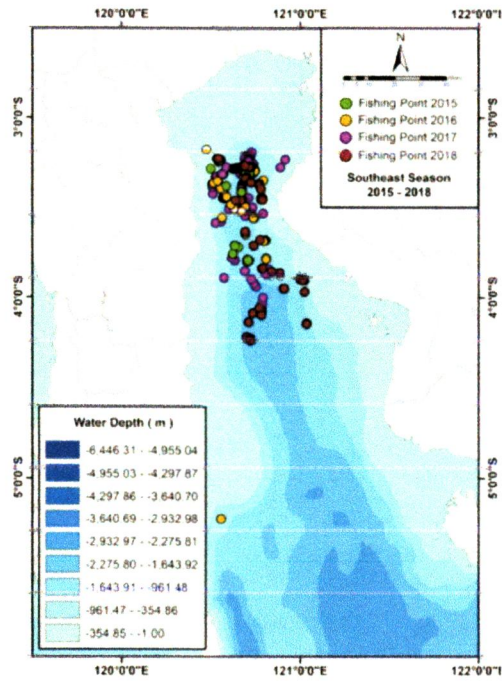
Figure 4. The profiles of bathymetric overlay with the skipjack tuna distribution during southeast monsoon from 2015 to 2018 in the Bone Gulf waters
