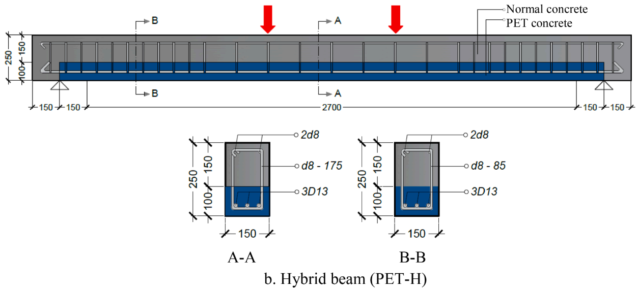
Fig. 4. Details of specimens.
