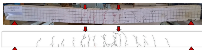
Fig. 12. Crack pattern of CB.
