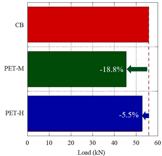
Fig. 11. Strength reduction.
