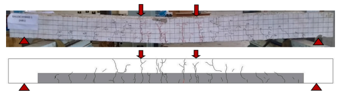
Fig. 13. Crack pattern of PET-H.
