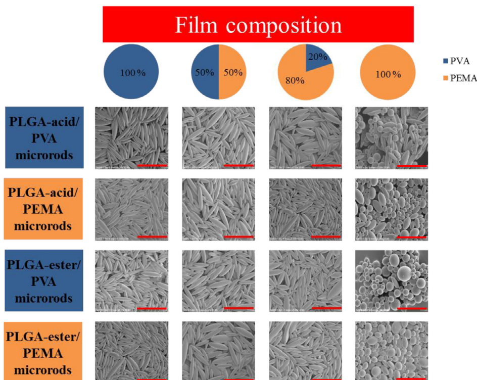
Fig. 2 – SEM images of microrods fabricated using different proportions of PEMA and PVA with four differently formulated microspheres. The scale bars are 10 µm.
