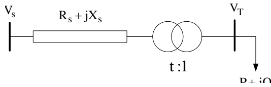
Figure 3: Model Thevenin Equivalent
