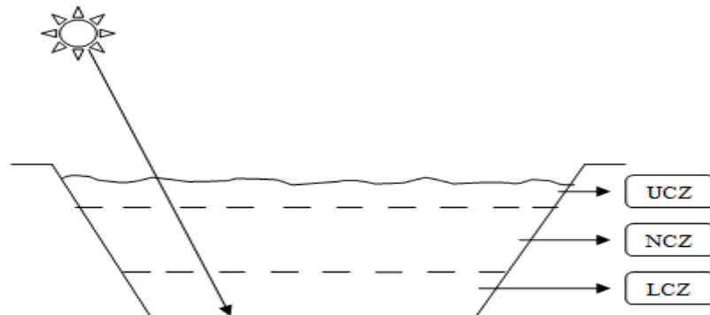
Figure 1. Solar Pond layer modeling
