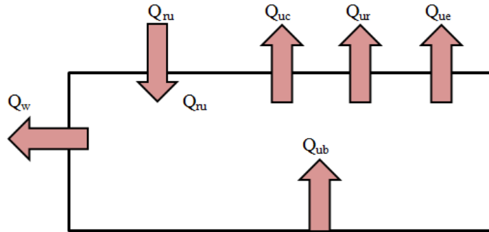
Figure 3. Heat Balance On Upper Zone
