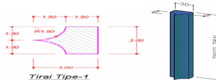
Figure-3. Shape Curtain Rectanguler with Wedge Shape Curve (Rwwsc).
