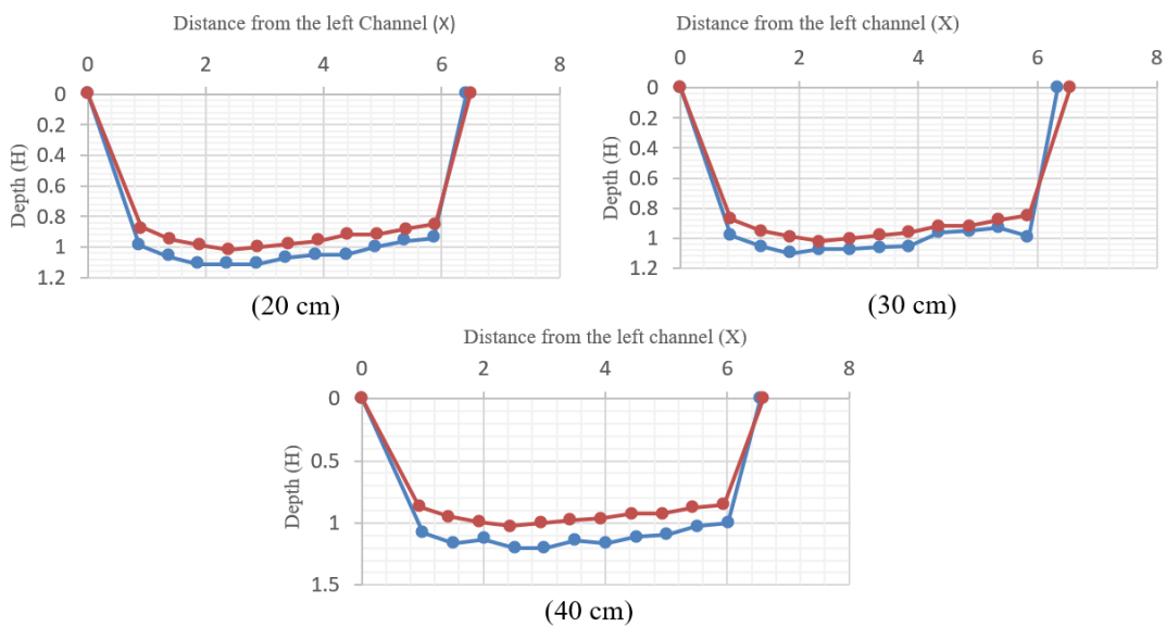
Figure 6. Channel transverse profile in stone pair channel.
