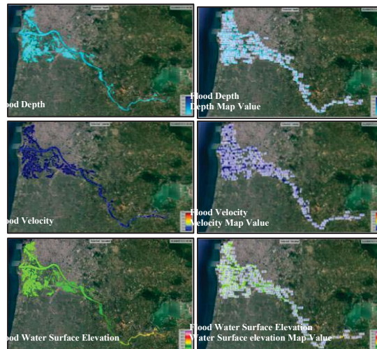
FIGURE 7. Simulation of HEC-RAS Flood (RAS-MAPPER)
