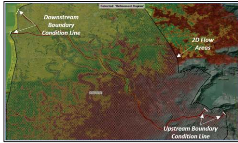
FIGURE 4. Element In the Simulation of Flood HEC-RAS
