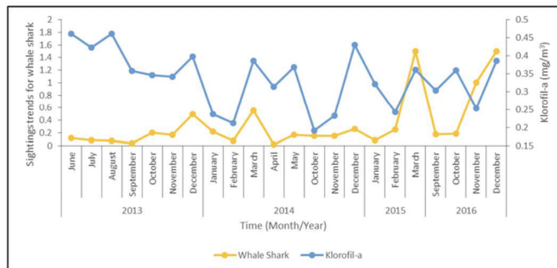
Figure 2: Temporal relationship between whale shark sightings and chlorophyll-a concentration (adapted from [4])
