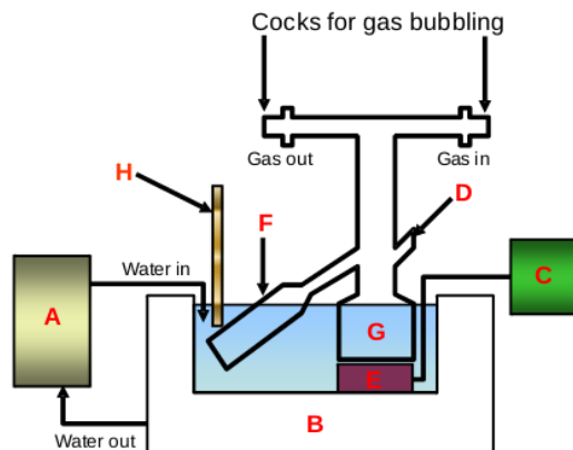
Fig. 1. Schematic view of the ultrasonic irradiation system.
