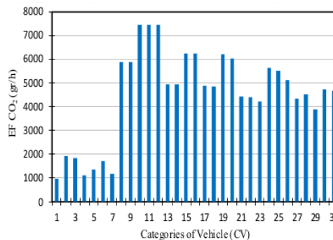
Fig.5 CO 2 EFs for 31 CV
