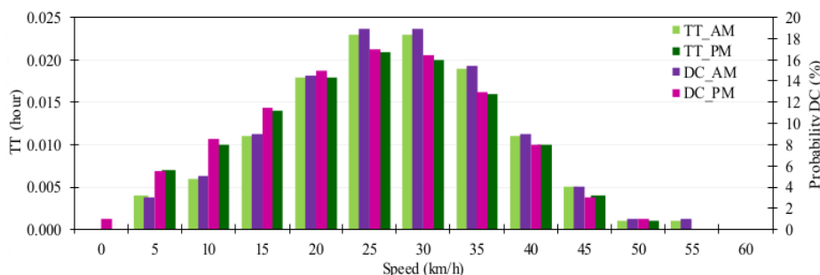
Fig.4 Speed, driving cycle, and TT
