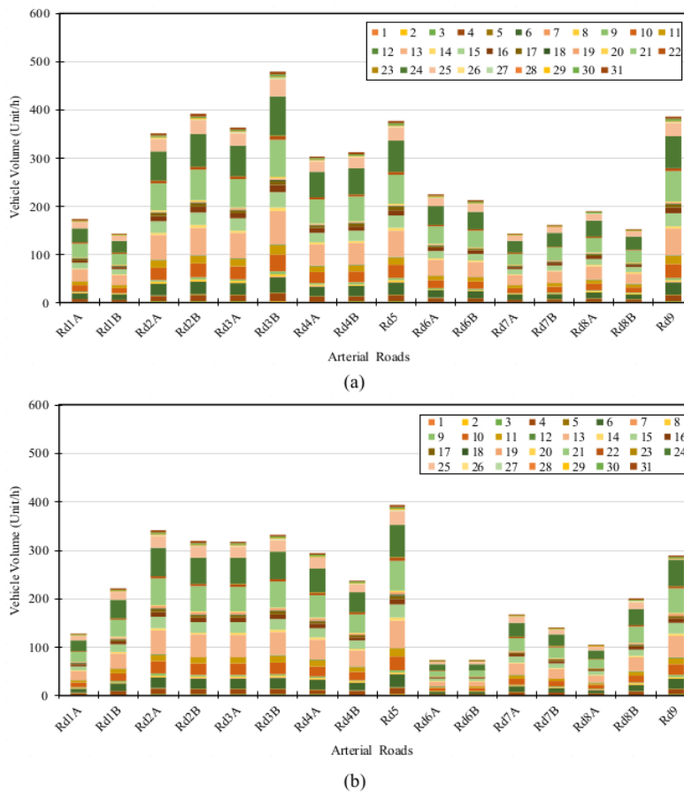
Fig.3 Vehicle Volume on Arterial Roads based on 31 categories of vehicles (CV). (a) Vehicle Volume on the morning (b) Vehicle Volume on the afternoon
