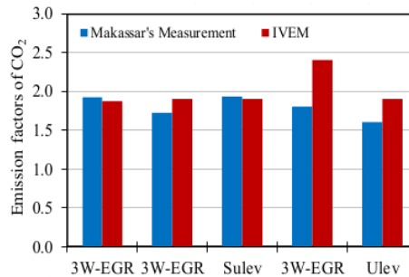
Fig.2 EF of Marni Model and IVEM
