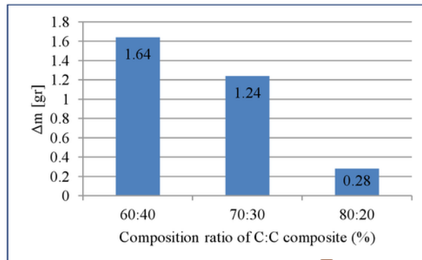
Figure 4. Graph of attrition testing result for C/C composites.
