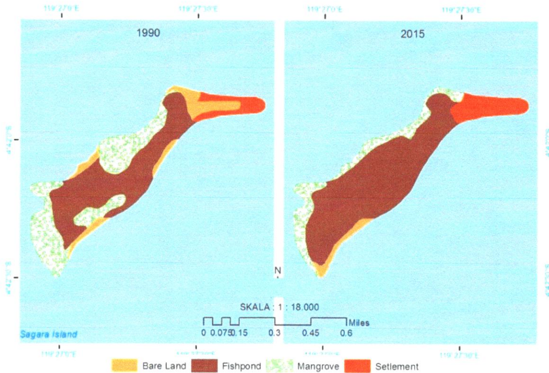
Figure 2. Mangrove classification maps in 1990 and 2015
