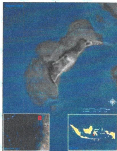
Figure 1. Sagara island is one of the small islands in Spermonde Archipelago, Indonesia as study area
