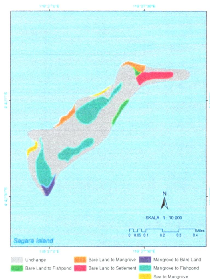
Figure 3. Post classification of mangrove in Sagara island of 1990 to 2015
