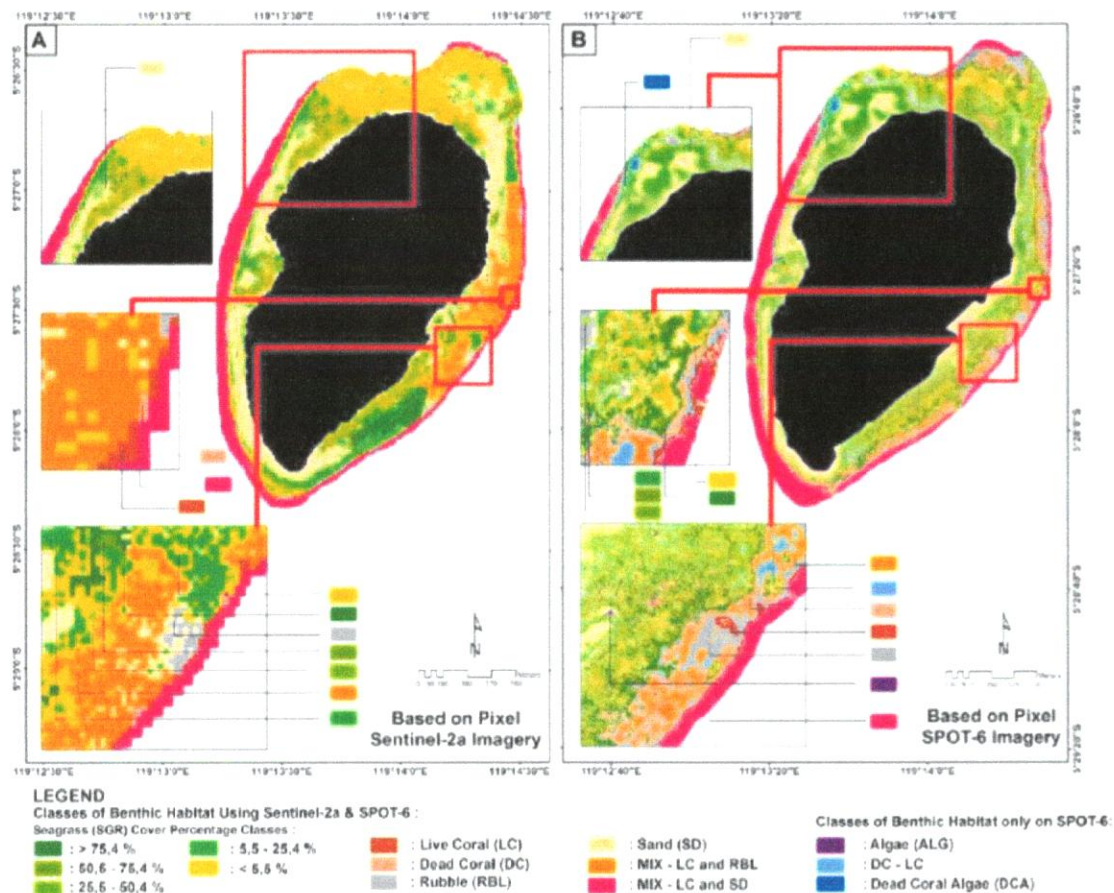
Figure 3. Result classification with the based on pixel. A) Classification based on pixel using Sentinel-2a, B) Classification based on pixel using SPOT-6,
