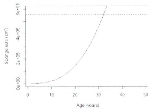
Figure 3. Model averaged size-at-age for all models combined. The dashed line represents the largest sponge volume recorded in this study (552,937.89 cm 3 ).
