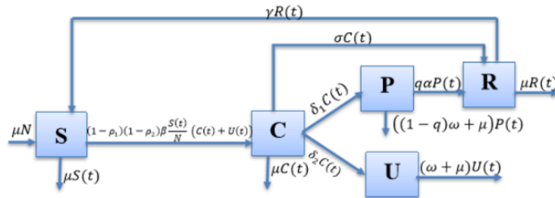
11 Figure 1. Transmission diagram of the mathematical model of the spread of COVID-19
