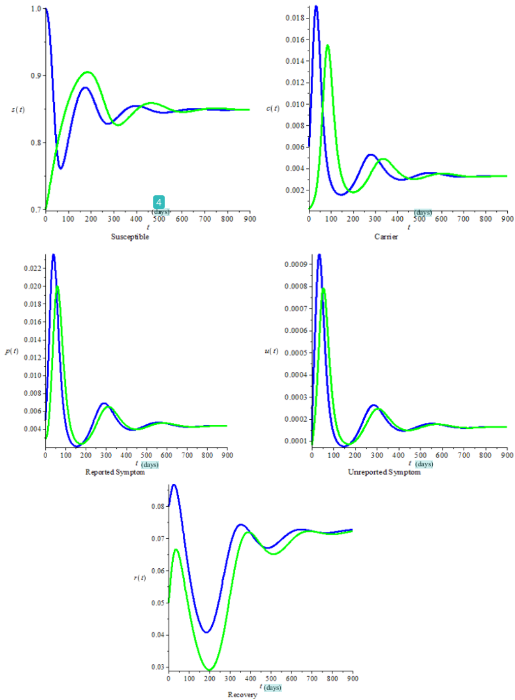
Figure 5. Graph of population when \beta = 0.65
