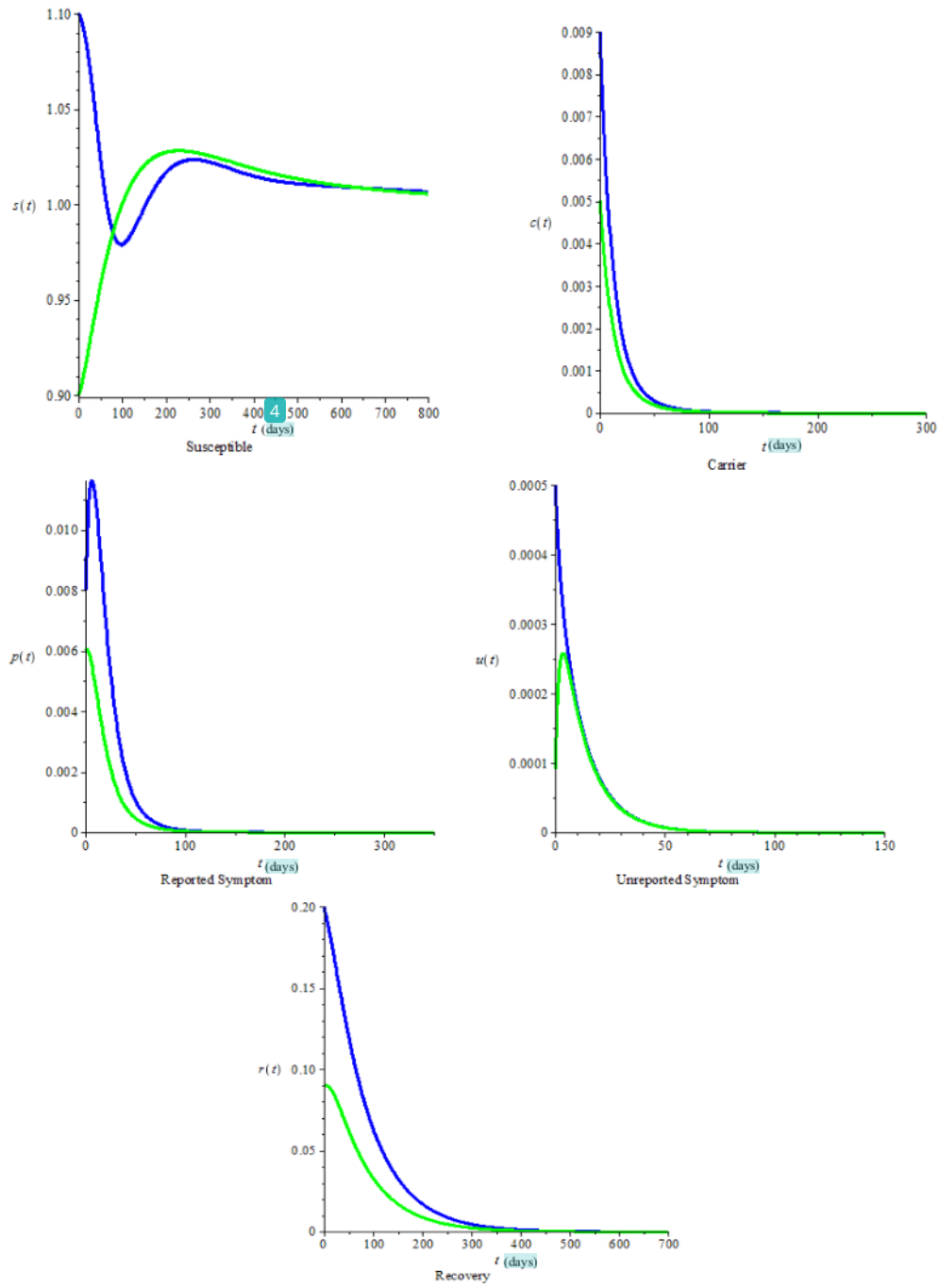
Figure 4. Graph of population when \rho_2 = 0.3423
