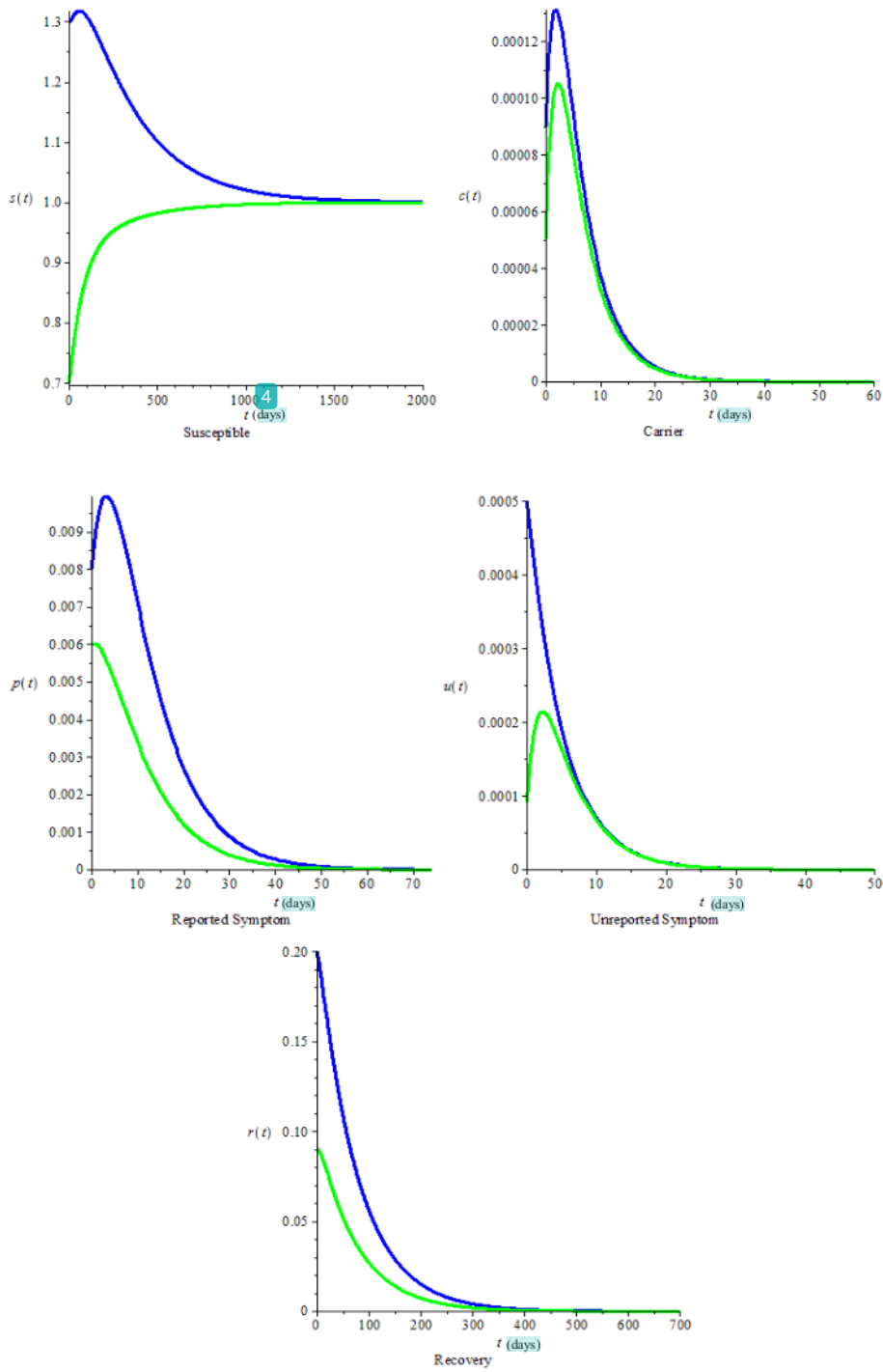
Figure 6. Graph of population when \beta = 0.3
