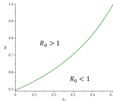
Figure 2. Relational function between \beta and \rho_2 when R_0 = 1
