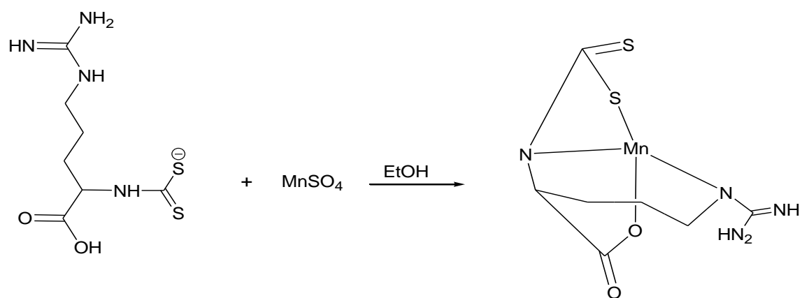
Figure 1. Synthesis reaction of Mn (II) arginine dithiocarbamate
