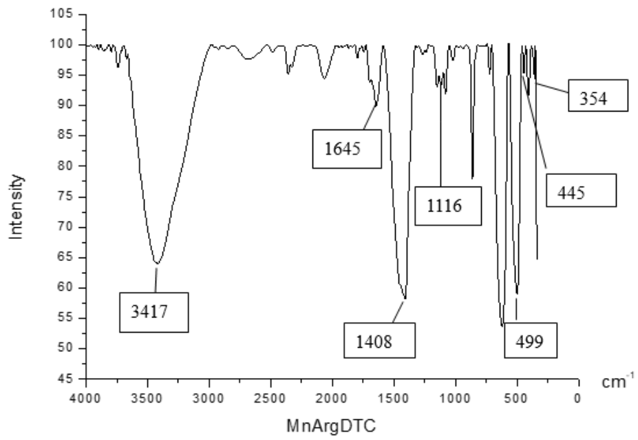
Figure 3. IR Spectrum of Mn (II) arginine dithiocarbamate
