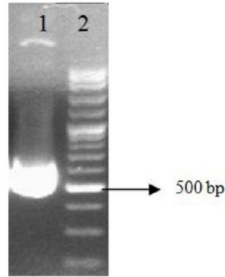
Figure 5. PCR analysis: 1) Rv 2430c :597bp 2) Marker 100 bp
