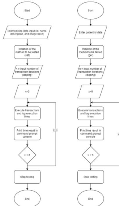
Fig. 5. Collecting Data Diagram Scenario.
