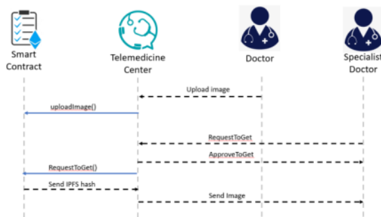
Fig. 2. Sequence Diagram for Blockchain Implementation.
