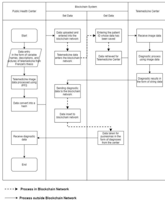
Fig. 1. Activity Diagram for Blockchain Implementation.
