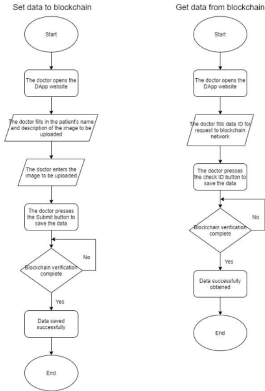
Fig. 4. Get and Set Function Scenario.
