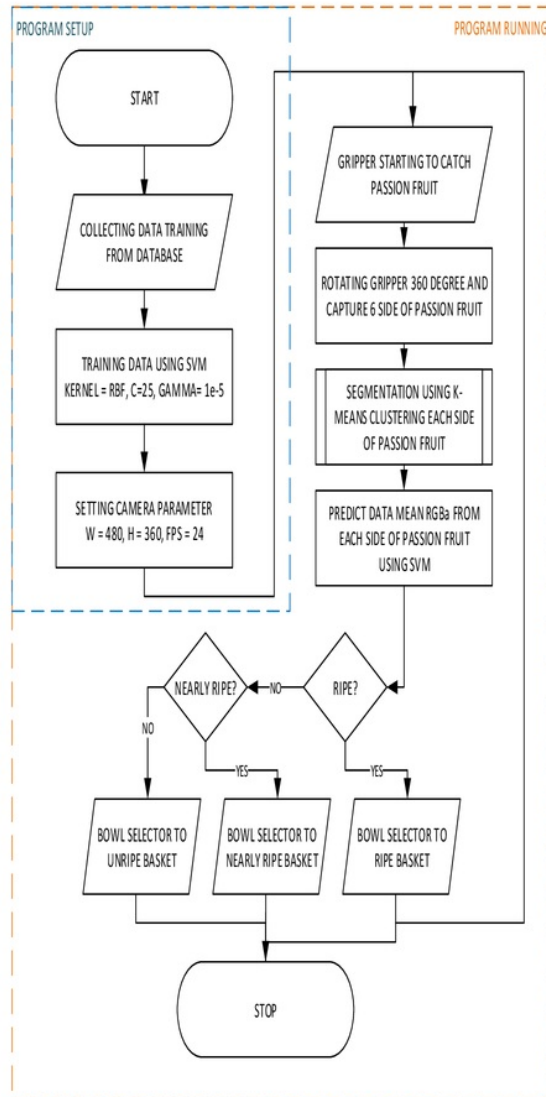
Fig. 4. Working Principles of Passion Fruit Sorting System
