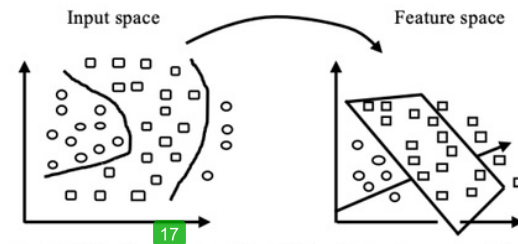
Fig. 3. SVMs allow mapping of the data from the input space to a high dimensional feature space by using Kernel Function
