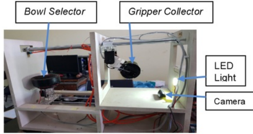
Fig. 9. Display all of Passion Fruit Sorting Machine
