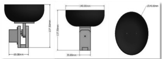
Fig. 8. Dimensions of the Bowl Selector
