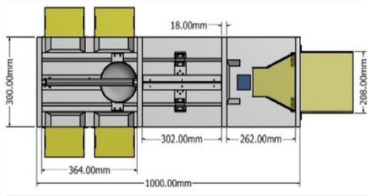
Fig. 6. Dimensions of Passion Fruit Sorting Machine Parts
