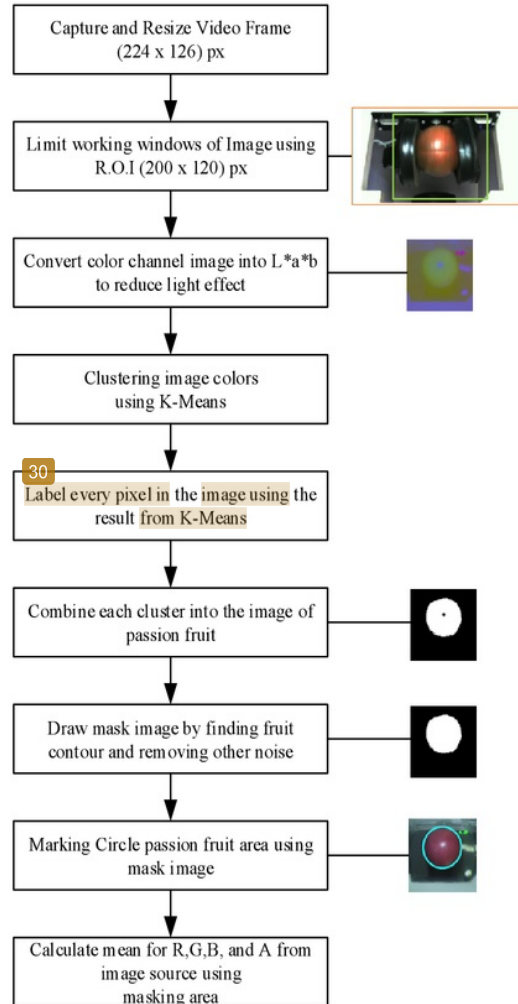
Fig. 2. The Process of K-Means Clustering Segmentation System
