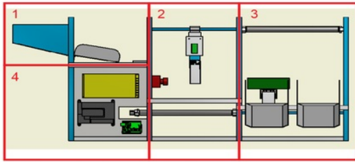
Fig. 5. Passion Fruit Sorting Machine Parts
