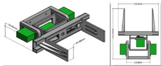
Fig. 7. Dimensions of the Gripper Collector
