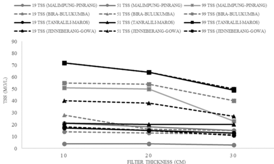
Fig. 5 Effect of filter thickness on TSS reduction
