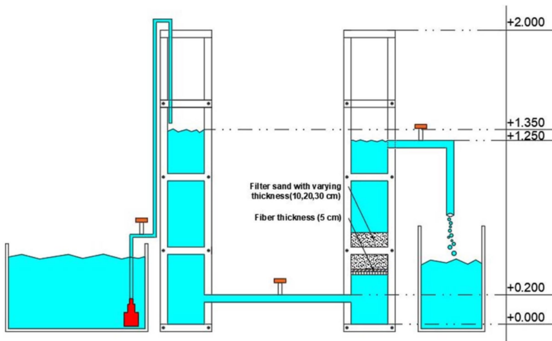
Fig. 1 The simulation equipment of the filtration process
