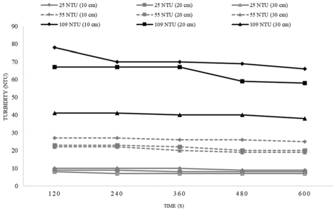
11 Fig. 6 The effect of time on the decrease in the NTU of Malimpung-Pinrang sand
