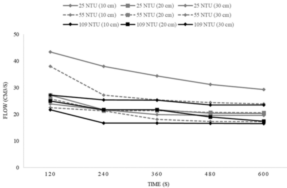
11 Fig. 7 The effect of time on changes of discharge in the Malimpung-Pinrang sand
