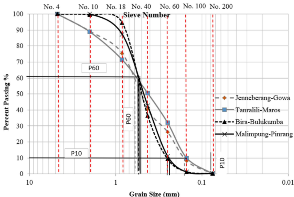
Fig. 3 Sieve analysis results
