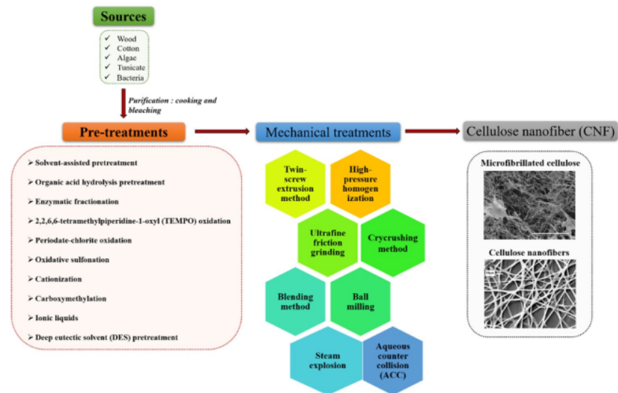
Fig. 3 Schematic representation of CNF preparation. SEM images of microfibrillated cellulose (reprinted with permission from [Henriksson et al. 2007]). SEM images of cellulose nanofibers (reprinted with permission from [Kim et al. 2006])
