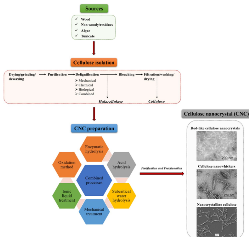
Fig. 2 Schematic representation of CNC preparation. Transmission electron microscopy (TEM) images of rod-like cellulose nanocrystals [reprinted with permission from (Li et al. 2018)]. Scanning electron microscopy (SEM) images of cellulose nanowhiskers [reprinted with permission from (Heath and Thielemans 2010)]. SEM images of nanocrystalline cellulose [reprinted with permission from (Anzlovar et al. 2018)]
