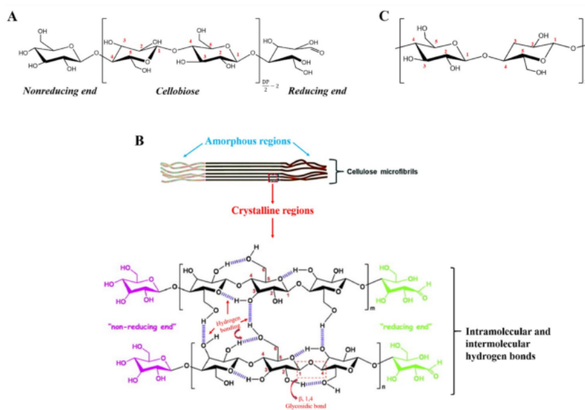
Fig. 1 a Chemical structures of CNC and CNF. b Intramolecular and intermolecular hydrogen bonds in crystalline cellulose [reproduced with modification from (Lin and Dufresne 2014)]. c Chemical structure of BC
