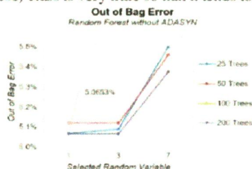
Figure 1. OOB of random forest model.
