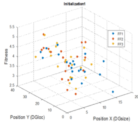
Fig. 3. Initialization Process.
