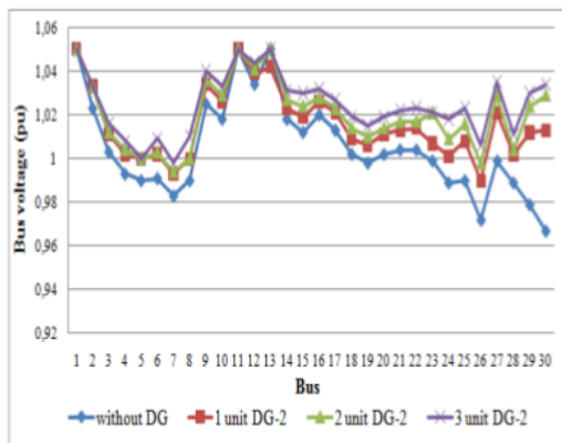
Fig. 6. Voltage Profile after DG-2 Placement.
