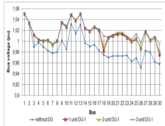
Fig. 5. Voltage Profile after DG-1 Placement.
