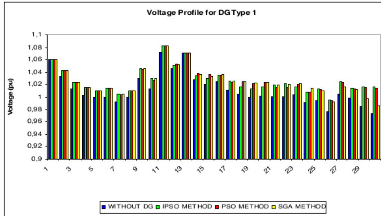
Figure 3: Voltage before and after DG type 1 installation
