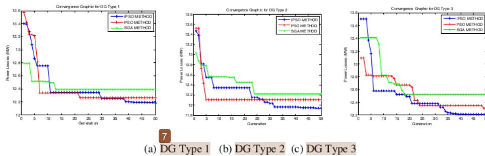
Figure 2: The Convergence Graphic Comparison of IPSO, PSO and SGA Methods
