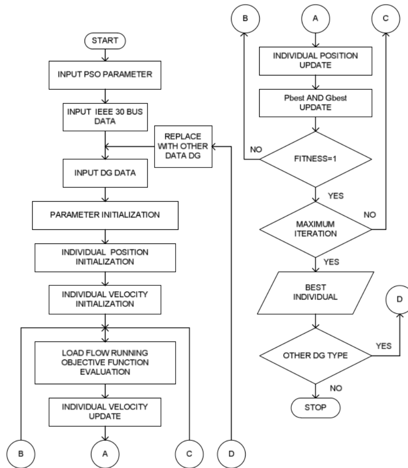
Figure 1: The optimization using IPSO method flow chart
