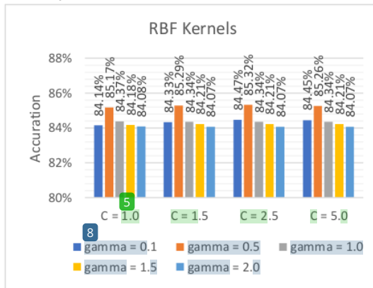
Fig 7. Comparison Graph of Accuracy based on Gamma and C values
