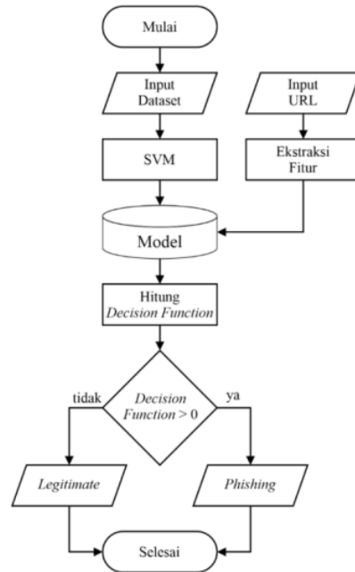
Fig 3. Flowchart of Implementation System
