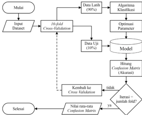
Fig 2. Evaluation System Flowchart
