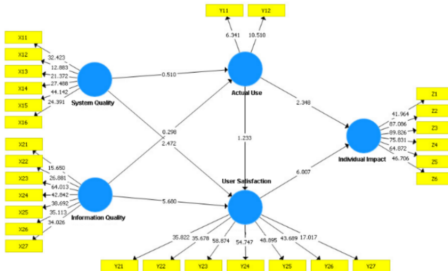
Figure 3. The 1st PLS Bootstrapping Model
