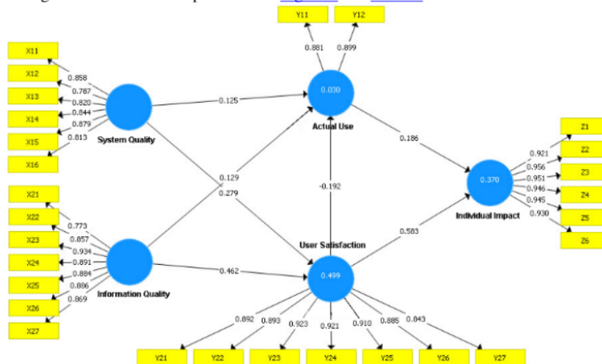
Figure 2. PLS Algorithm Model
