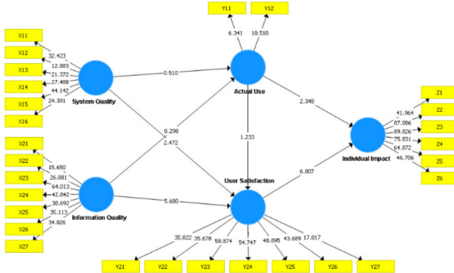
Figure 4. 2nd PLS Bootstrapping Model
