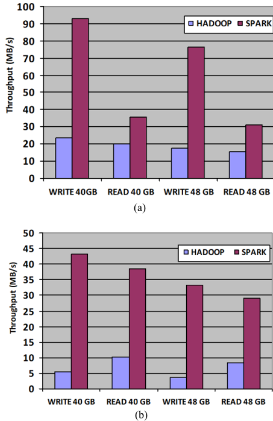
Figure 4 : TestDFSIO Throughput on the (a) Type 1 Cluster (b) Type 2 Cluster
