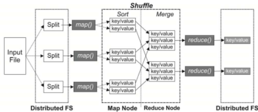
Figure 2: MapReduce Model
