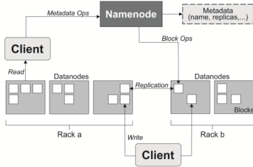
Figure 1: An HDFS Architecture
