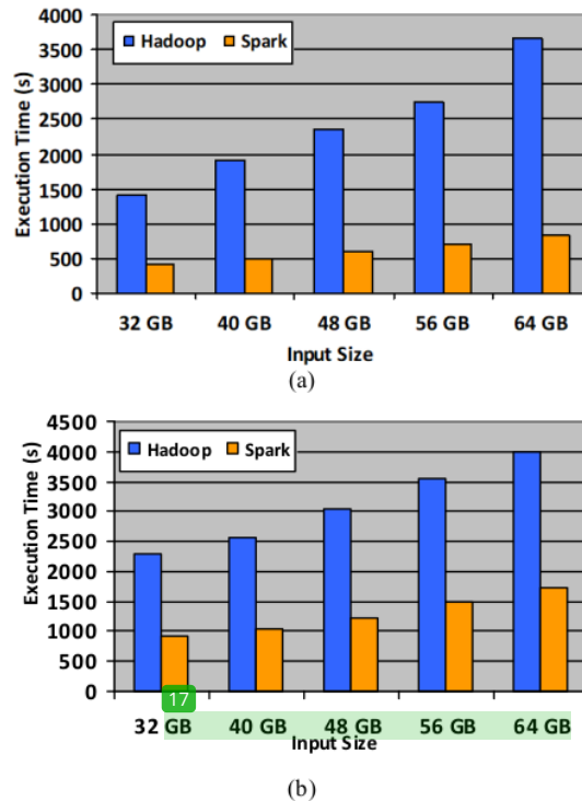
Figure 3 Wordcount Execution Time on the (a) Type 1 Cluster (b) Type 2 cluster
