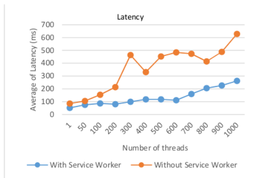
Fig. 5. Latency with and without Service Worker
