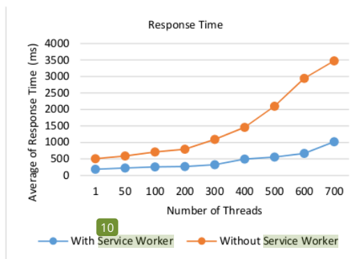
Fig. 3. Response time with and without Service Worker
