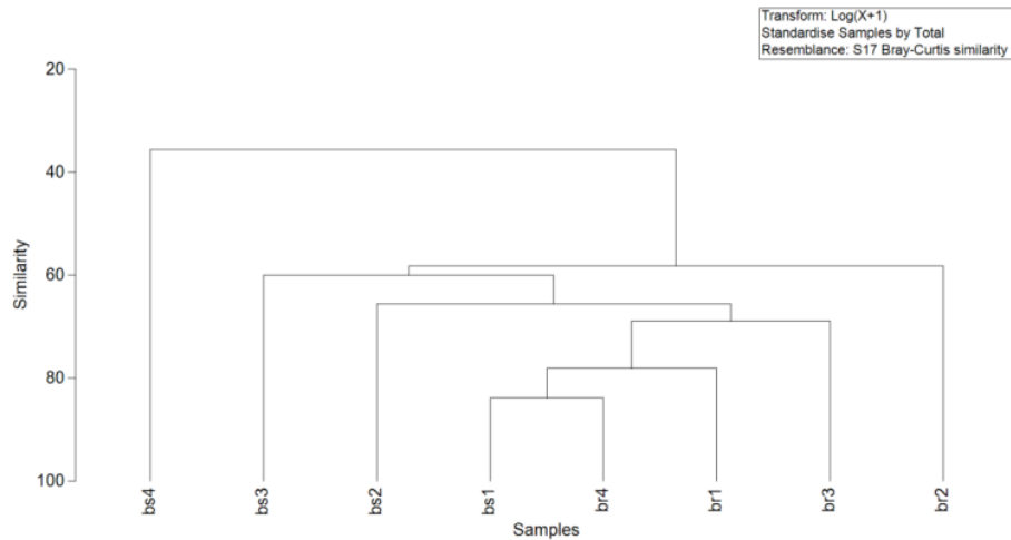
Figure 3. Analysis of similarity from eight sampling locations at the two river mouths of the Bengawan Solo and Brantas rivers in East Java
